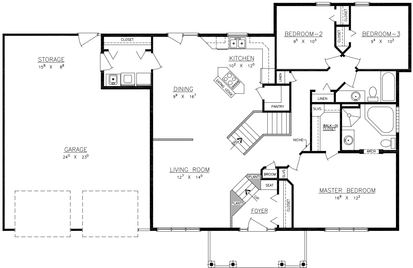
FLOOR PLAN
